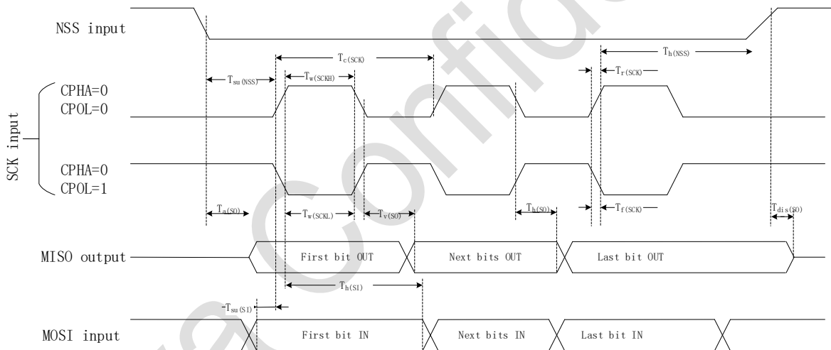
图 5-1 SPI 时序图—slave mode and CPHA=0
