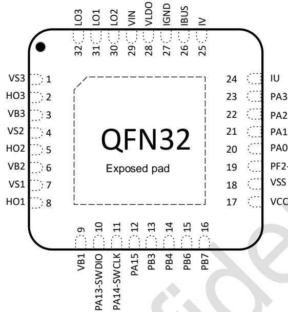
图 3-1 QFN32(4*4) Pinout1 PY32MD420K1xU
